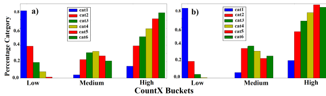
Figure 6: Correlating citation count and countX buckets. (a) Correlation at 5 years after publication; (b) Correlation at 9 years after publication
