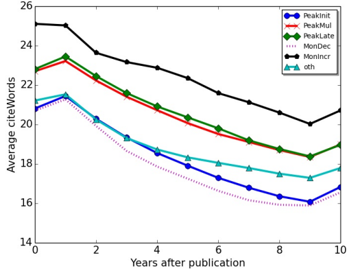
Figure 5: Average citeWords: temporal profiles for the six citation categories [6] over the first 10 years of publication age
