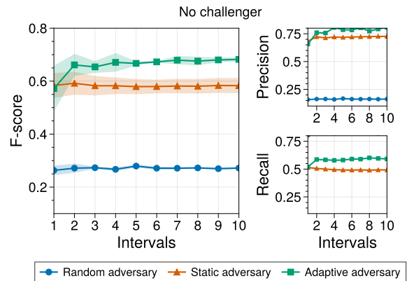
Fig. 5: F-score of different adversaries (random, static, adaptive) when no privacy preserving deletion mechanism is in place. No filtering based on the keywords of tweet were made. Shaded areas represent 95% confidence intervals.
