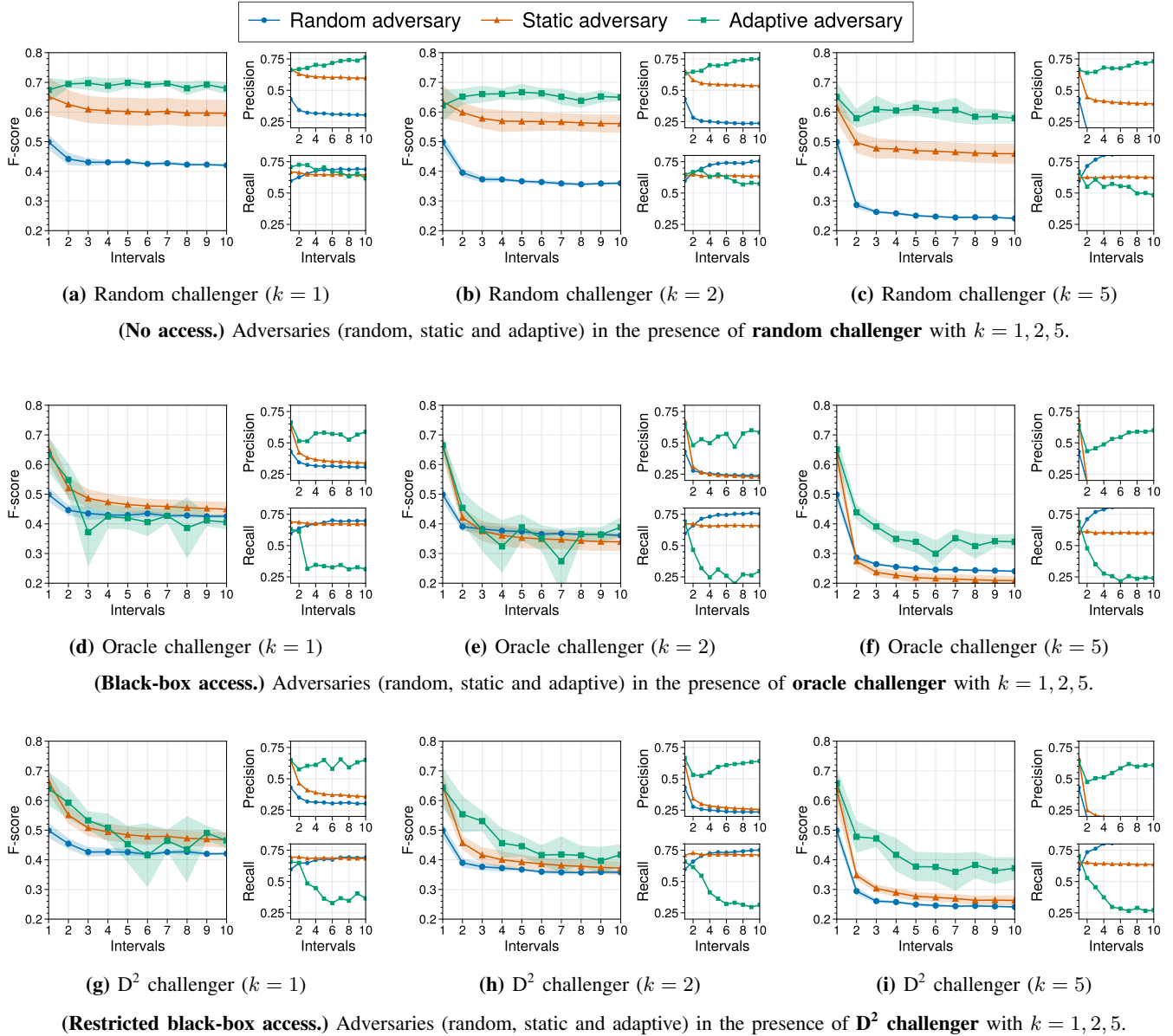
Fig. 4: F-score (with 95% confidence intervals), precision and recall for the three adversaries (random, static and adaptive) in the presence of different challengers corresponding to different accesses with k = 1, 2, 5 . Key observation: D^2 challenger fools the adversaries almost as well as the oracle challenger but with a restricted black-box access.
