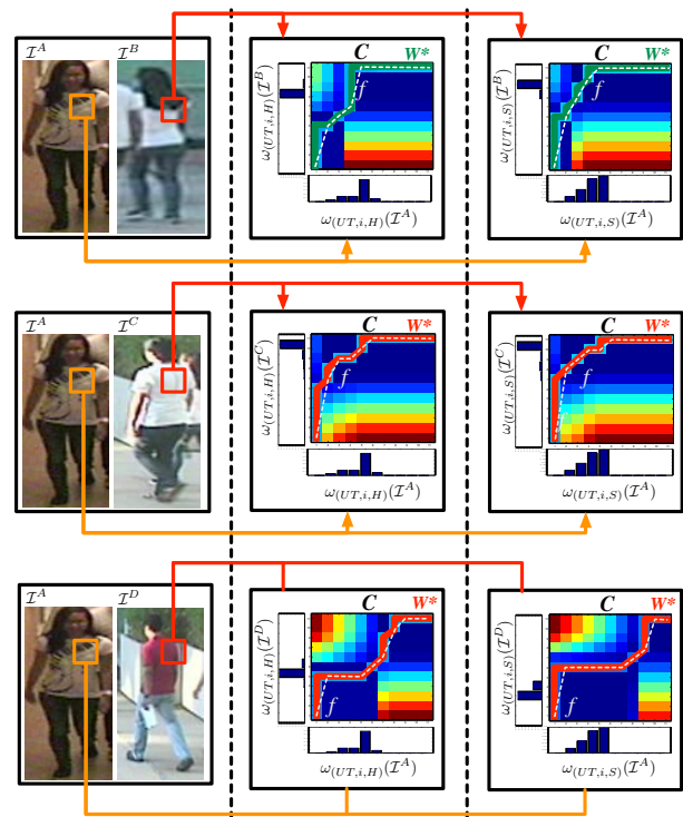
Fig. 7. Example of computing the warp functions between features extracted from the same patch of two images. The first column shows two images from two cameras. The warp function between the features extracted from the same patches (shown by the orange and red boxes) are computed next. The last two columns show the cost matrices, the optimal warp path W^* and the corresponding warp function f . For convenience of visualization, warp functions computed for the H and S colorspace only are shown in second and third column respectively. The cost matrix is color-coded and the cost gets higher as the color goes from blue to red. First row shows the feature warps for the same person. Second and third rows show the warping of features between different persons that have similar and different appearance respectively with the person in the left.
