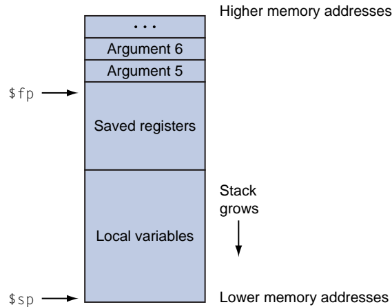
FIGURE A.6.2 Layout of a stack frame. The frame pointer ( \$fp ) points to the first word in the currently executing procedure's stack frame. The stack pointer ( \$sp ) points to the last word of frame. The first four arguments are passed in registers, so the fifth argument is the first one stored on the stack.
