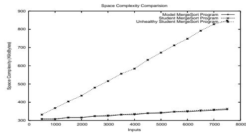
Figure 10: Space Complexity of MergeSort programs
