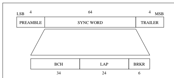
Figure 5: Channel Access Code
