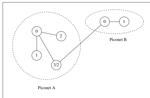
Figure 2: Scatternet Example
